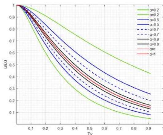
Figure 3 : Max excess pore pressure vs Time factor [21]
