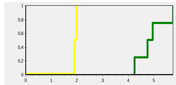
Figure 6 : Construction of Upper and Lower probabilities vs Number of soundings
