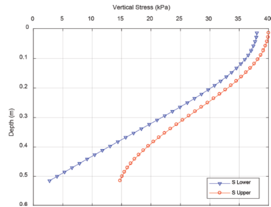
Figure 1 : Vertical stress distribution under axis for surficial pressure q and interval coefficient k
