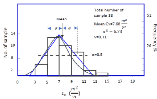
Figure 2 : Approximation of C_v by a fuzzy set [20]
